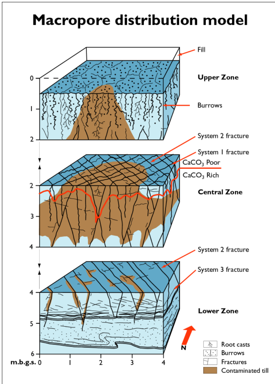
Figure 21. Model of the macropore/fracture systems in clayey tills (From Klint & Graven, 1994).
