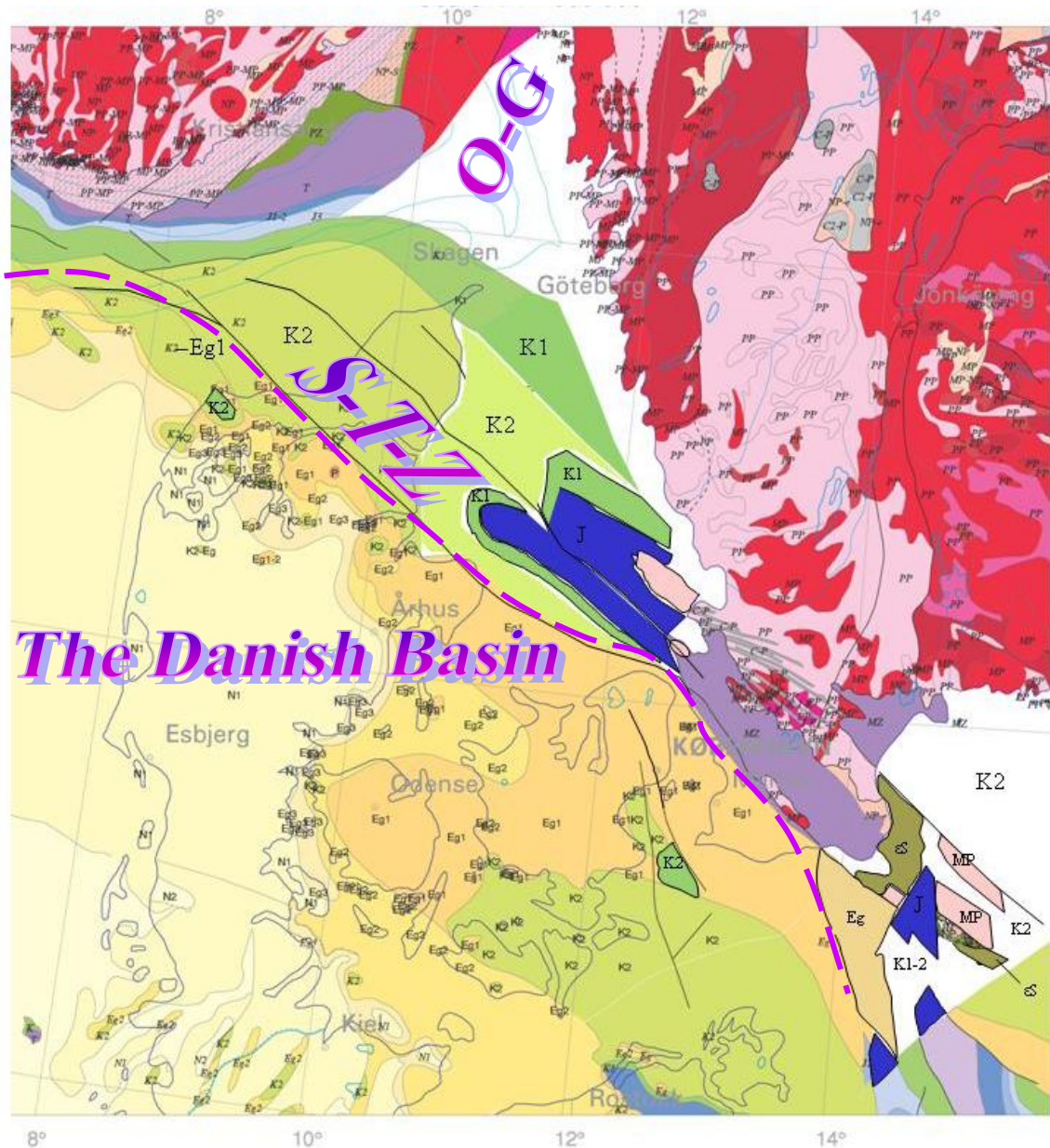
Figure 2. Pre-Quaternary map of Denmark. Red colours are Precambrian basement rocks at the margin of the Danish Basin. Blue colours are Jurassic and Triassic units, mainly occurring in fault blocks in the NW-SE striking Sorgenfrei-Tornquist Fault Zone (STZ). Green colours are Cretaceous chalk (K2), yellow-brown colour (EG1) is lower Tertiary limestone and marly clay. The light beige colour (N1) is Miocene sand deposits, which 15 million years ago formed a huge delta setting for the rivers draining the mainland of Europe out towards the North Sea. Between EG1 and N1, a number of clayey units appear mirroring the marine conditions under fluctuating water levels. O-G is the Oslo Graben, which is characterized by Permian volcanics. (Modified from Pedersen et al., 2002 and Pedersen, 2009).
