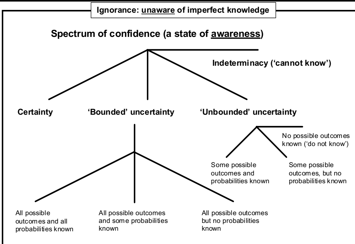
Fig. 33 Taxonomy of imperfect knowledge resulting in different uncertainty situations (Brown, 2004)
