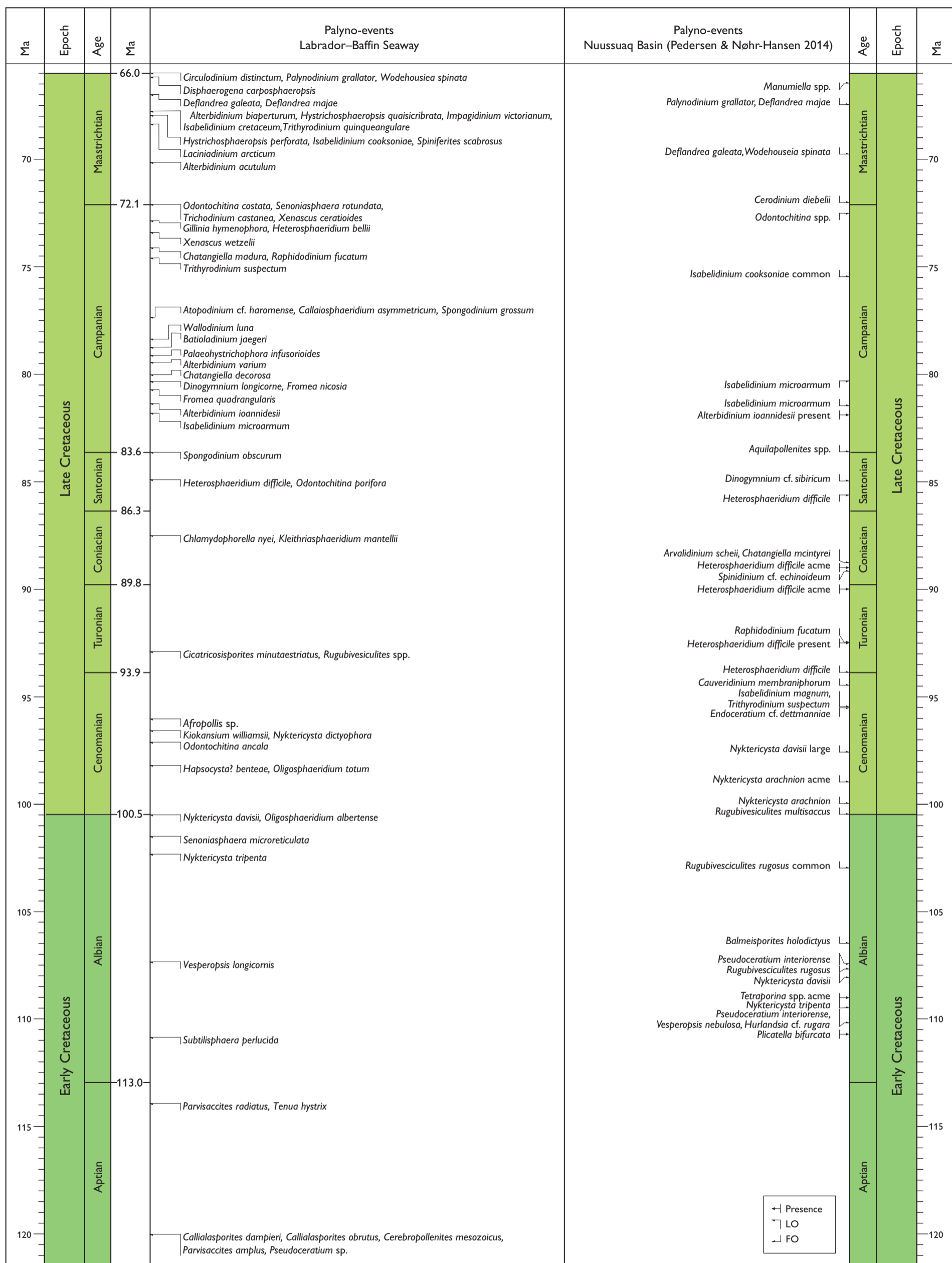
Fig. 5. Key palynostratigraphic events in Cretaceous strata of the Labrador–Baffin Seaway and adjacent areas. The events from the seaway are exclusively ‘Last Occurrences’ (LO), whereas the Nuussuaq Basin events also include ‘First Occurrences’ (FO). Systematic palynology of the assemblages, including new taxa, is presented herein; timescale (Ma) from Gradstein et al. (2012).
